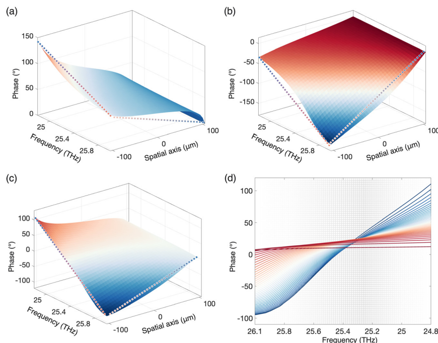
Fig. 3 An example of creating a linear phase function in frequency and space for the proposed dual band color-sorter. (a) Phase function of an array of Huygens' resonances with tuned damping. (b) Phase function of another one-dimensionally aligned Huygens' resonance at an adjacent frequency. Neither of the functions in (a) and (b) is linear in frequency and space. (c) The sum of the functions in (a) and (b) displays an improved linearity. (d) The projection of the function in (c) onto the frequency-phase axis.
