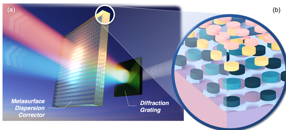
Fig. 1 A schematic of the proposed dual-band color-sorter design. A broadband signal (white color, on the right side of (a)) is spread by a grating and then binned into two discrete angles for each band (pink and blue colors on the left side of (a)) as it passes through the metasurface dispersion corrector. The metasurface can be fabricated on top of the grating. Here they are separated for convenience. (b) A zoom-in view that illustrates multi-layer disk-shaped nano-resonators in the dielectric metasurface.
