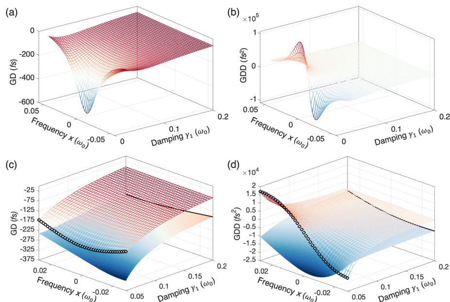
Fig. 2 The group delay (GD) and group delay dispersion (GDD) of a Huygens' resonance. (a) and (b) GD and GDD of a single Huygens' resonance. (c) and (d) Comparison of the GD and GDD of paired Huygens' resonances (solid surfaces) to parts of (a) and (b) (mesh surface). The paired resonances produce the same GD with a much smaller GDD. The resonance offset parameter \delta and damping parameter \gamma_2 are set to 0.06 and 0.1, respectively.
