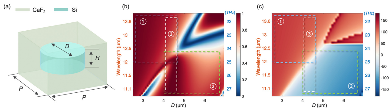
Fig. 4 (a) A schematic of a band sorter metasurface unit cell with a silicon ( n = 3.41 ) disk embedded in a \text{CaF}_2 ( n = 1.23 ) substrate. (b) The transmittance of a unit cell. The high transmittance region where the three dashed boxes overlap indicates the excitation of a Huygens' dipole mode. The dashed boxes 1–3 mark the regions of high transmittance that are used in our design. The boxes of the same index in (c) mark the corresponding phase responses. (b) and (c): axes on the right (blue) show frequencies corresponding to the wavelengths on the left (orange).
