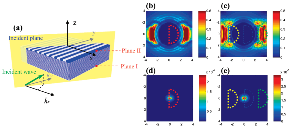
Figure 3. Two-dimensional transfer functions of a metamaterial FSL (the metamaterial FSL is made of 20 pairs of 15 nm Ag/20 nm dielectric ( \epsilon = 2.28 ) and a 1D Ag–dielectric subwavelength grating. The thickness, period, and Ag filling ratio of the subwavelength grating are 55 nm, 160 nm, and 0.3, respectively. The working wavelength is 405 nm). (a) Schematic of the incident wave with respect to the metamaterial FSL. (b,c) Zero and first-order transfer function for p-polarization. (d,e) Zero and first-order transfer function for s-polarization. The unit in both horizontal and vertical axis are k_0 . Notice the color scale difference between (b,c) and (d,e).
