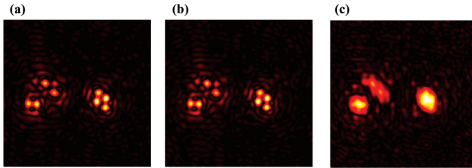
Figure 5. Image reconstructed at wavelength (a) 500 nm, (b) 600 nm, and (c) 365 nm. The metamaterial FSLs and the objects are the same as those in Figure 4 except that the objects and the periods of the gratings in the metamaterial FSLs are scaled by the ratio of wavelengths (for example, at wavelength 500 nm, the object is scaled by the factor 500/405, and the period of the grating is changed from 160 to 200 nm). At wavelength 365 nm, the object can not be correctly reconstructed because the transmissions of the evanescent waves through the multilayer are comparable with those of the propagating waves.
