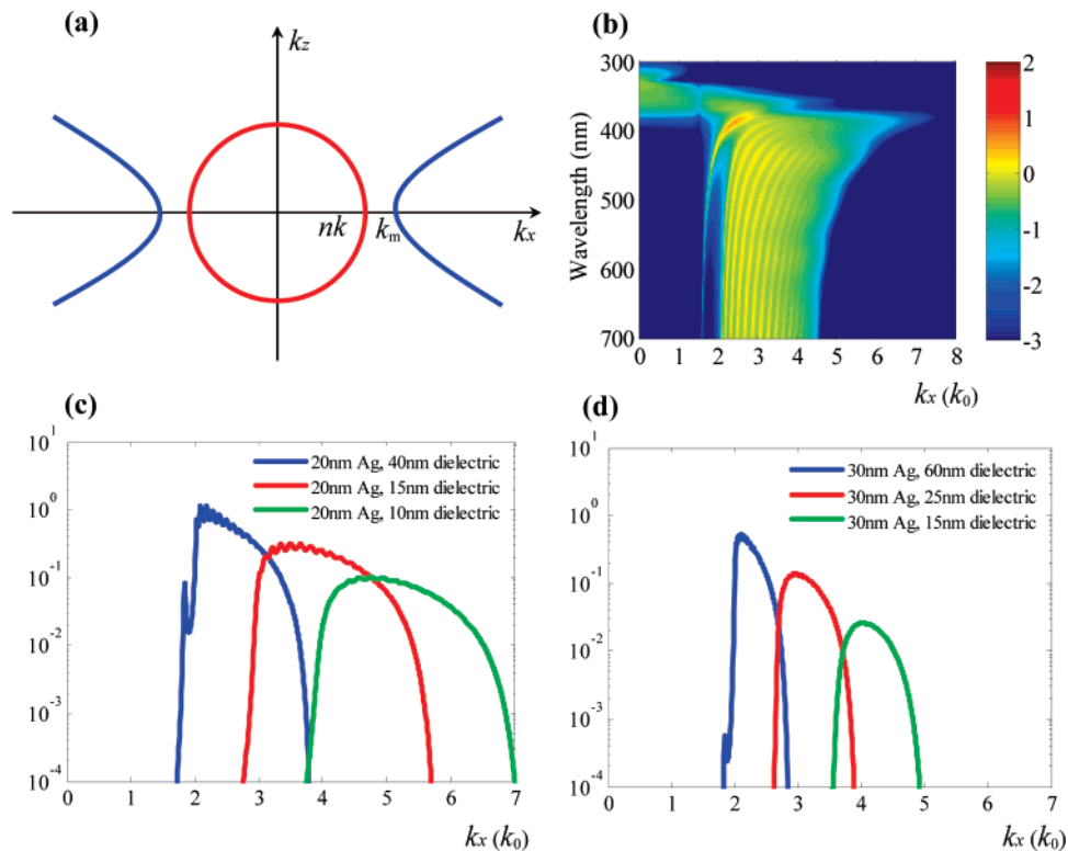
Figure 2. (a) Dispersion relation of a metal–dielectric multilayer with \epsilon_{\text{eff},z} > 0 , \epsilon_{\text{eff},x} < 0 . (b) Calculated transmission coefficients (in logarithm scale) of 20 pairs of 15 nm Ag and 20 nm dielectric multilayer. Permittivity of Ag is obtained from ref 24, while permittivity of dielectric is 2.28. (c) Calculated transmission coefficients (in logarithm scale) of 30 pairs of Ag (thickness of each Ag layer is 20 nm) and dielectric (wavelength is 450 nm). (d) Calculated transmission coefficients (in logarithm scale) of 30 pairs of Ag (thickness of each Ag layer is 30 nm) and dielectric (wavelength is 450 nm).
